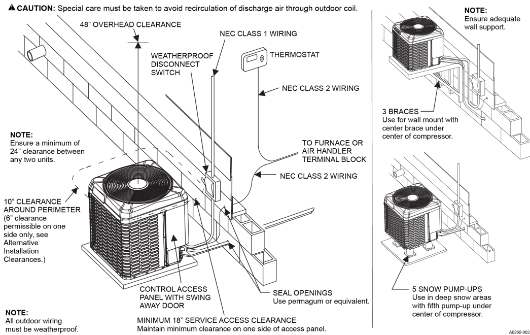
Figure 3: Typical installation
